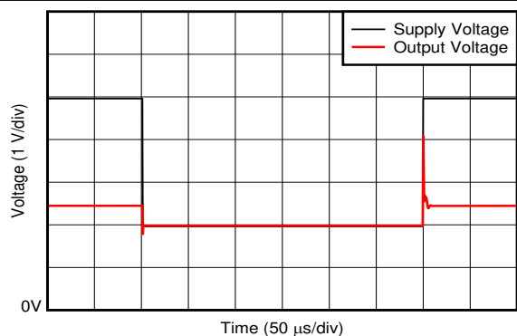
Figure 6-34. Supply Transient Response
